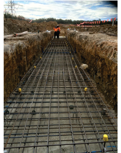
Slab prep for precast culvert units
